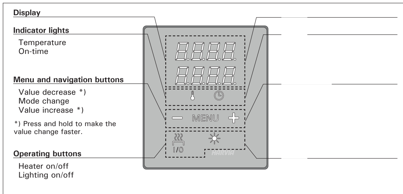
Figure 2. Control panel
