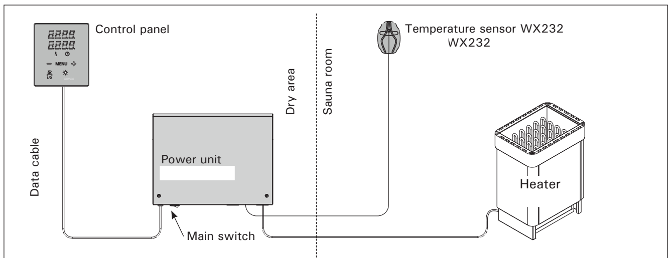
Figure 1. System components
