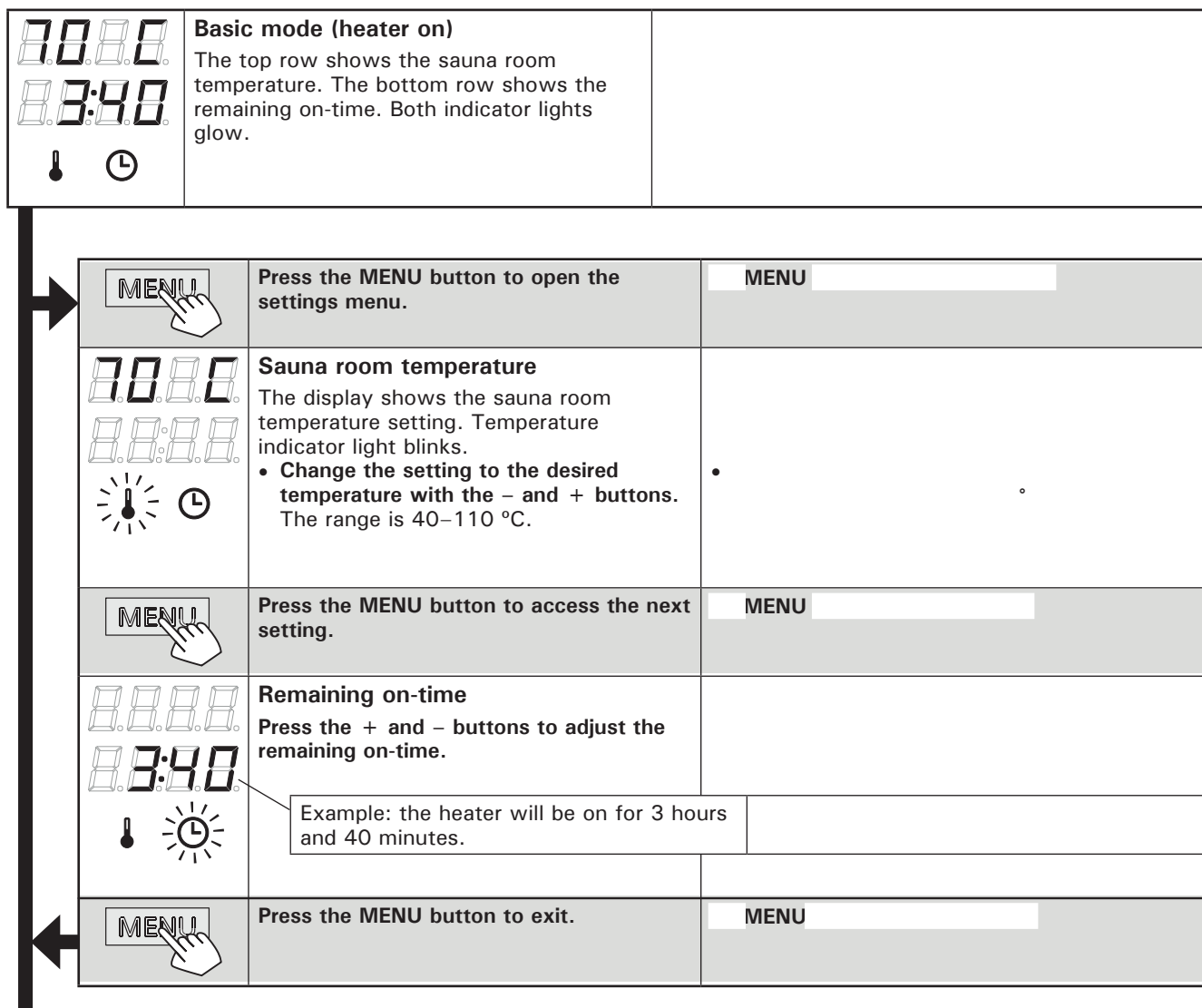
Figure 3a. Settings menu structure, basic settings
