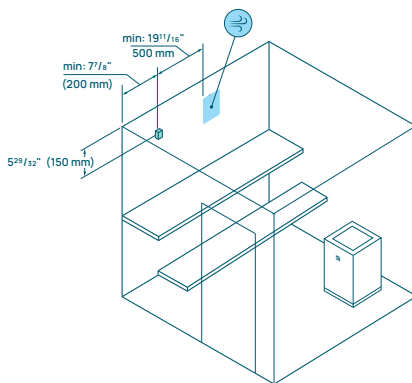
Figure 8. Bench sensor position from the corner, opening and ceiling
