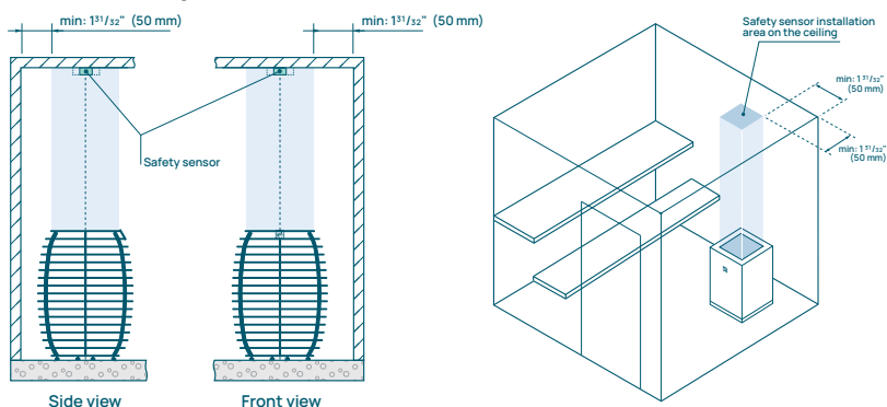
Figure 4. Installing the safety sensor: floor-mounted heater
