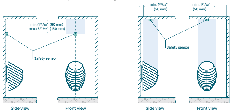
Figure 5. Installing the safety sensor on the wall: wall-mounted heater
