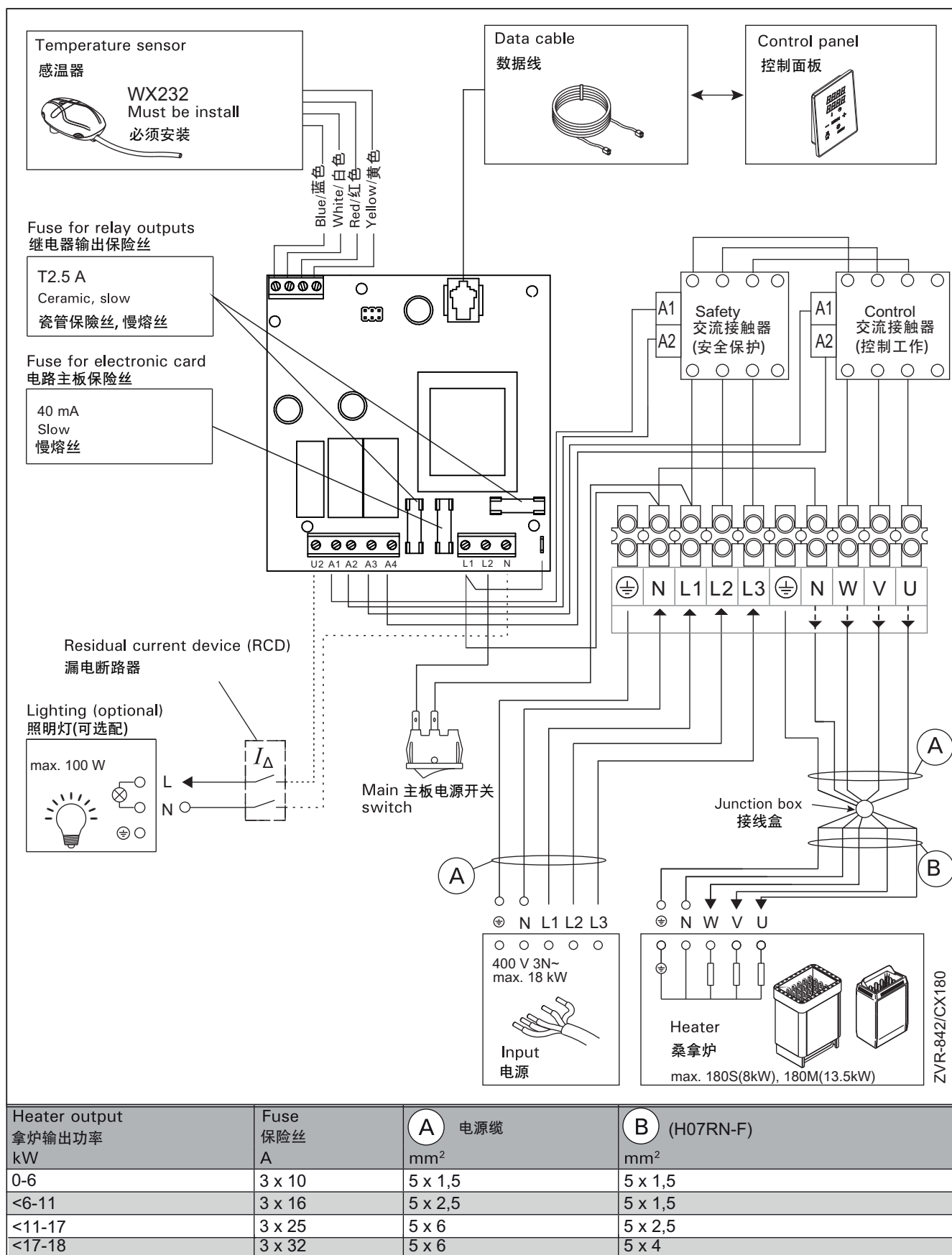
Figure 6a. CX180S, CX180M Electrical connections 图6a. CX180S, CX180M接线图
