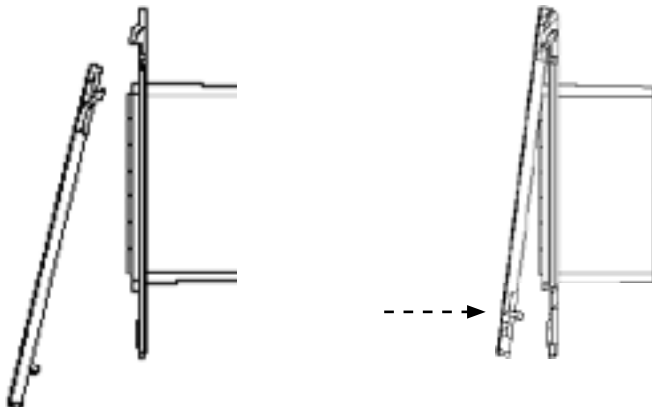
Abb. 4: Montage Frontcover
