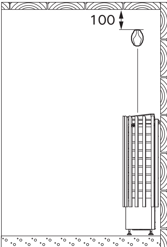
Installing the sensor (all dimensions in millimeters)
