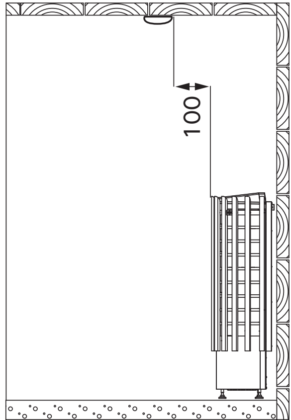
Installing the sensor (all dimensions in millimeters)
