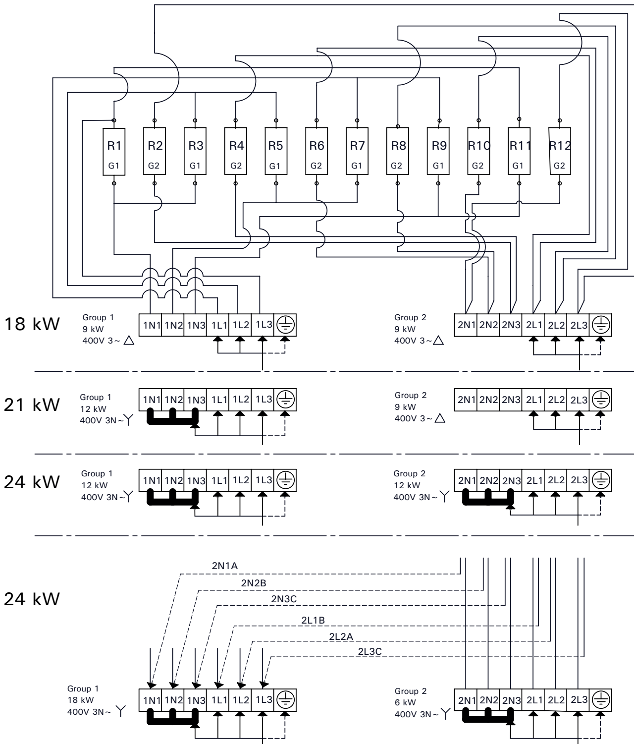
Figure 8. Electrical connections Abbildung 8. Elektroanschlüsse des Saunaofens
